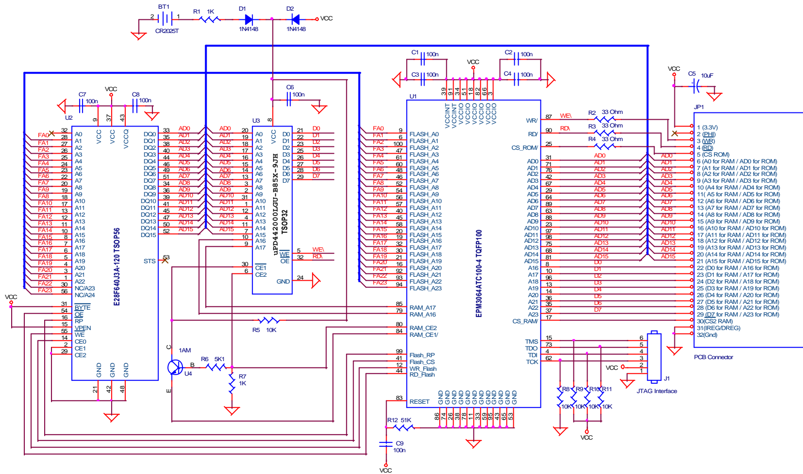
Flash cart for E28F320J3A-110 or E28F640J3A-120 and also larger chips. (C) 2002 by Reiner Ziegler ( www.reinerziegler.de )
